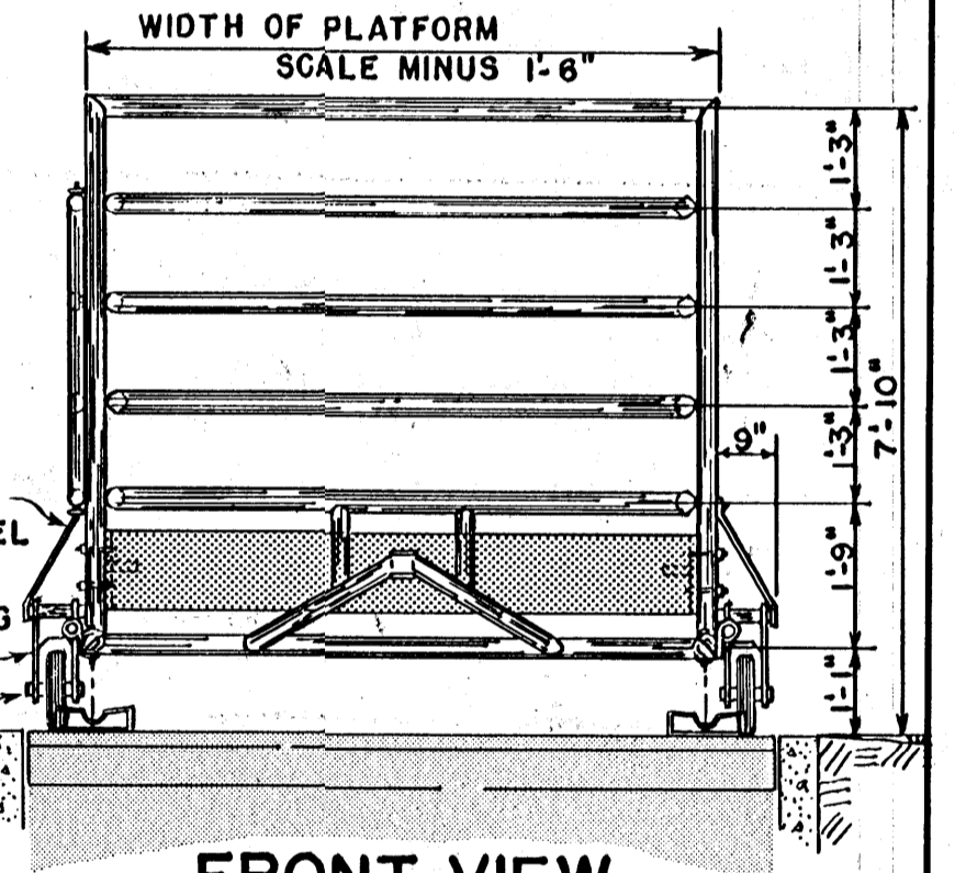
FRONT VIEW
