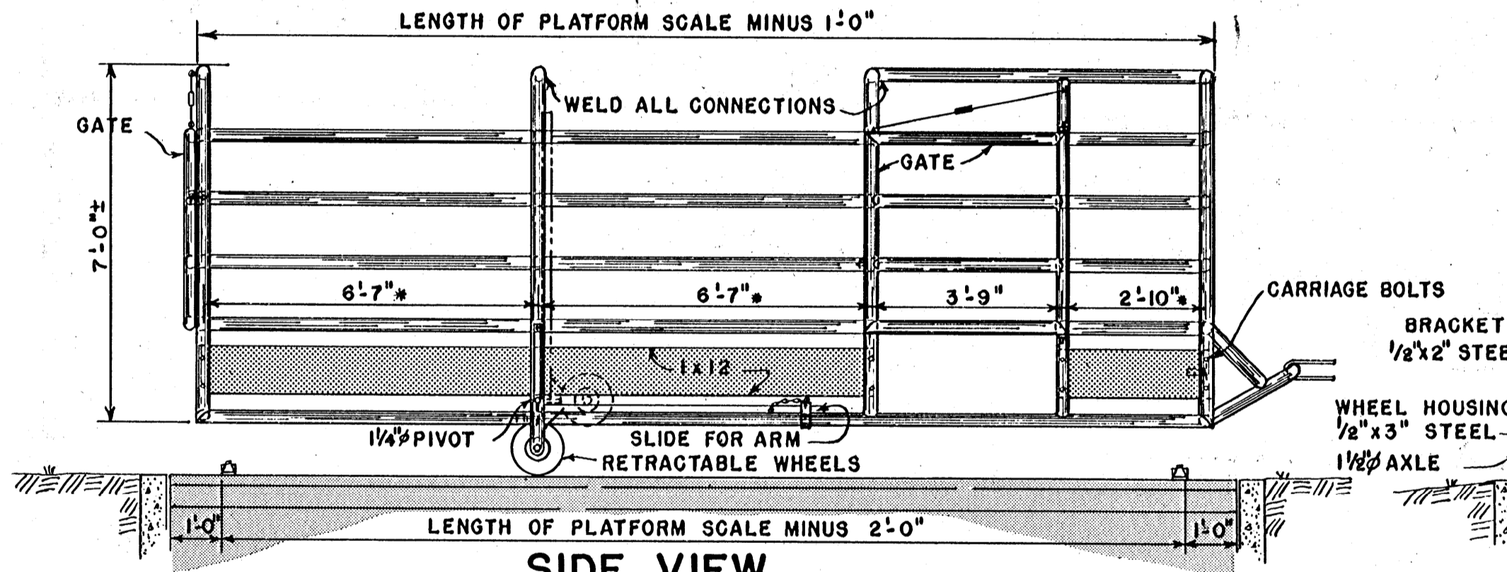
SIDE VIEW
