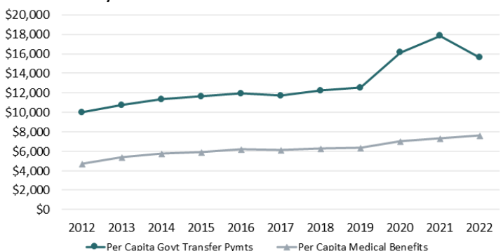
Per Capita Govt Transfer Payments and Medical Benefits Transfer Payments Noxubee County
