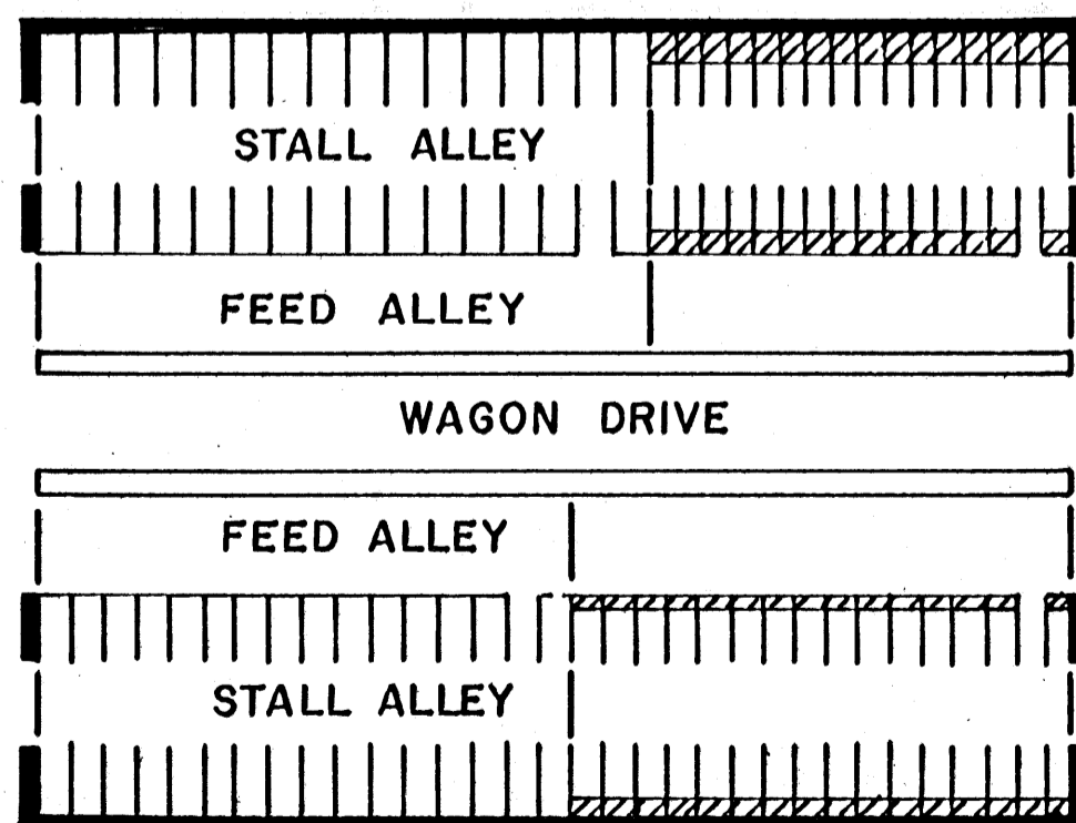
FIG. 6 - DOUBLE BARN FOR LARGE OPERATION
