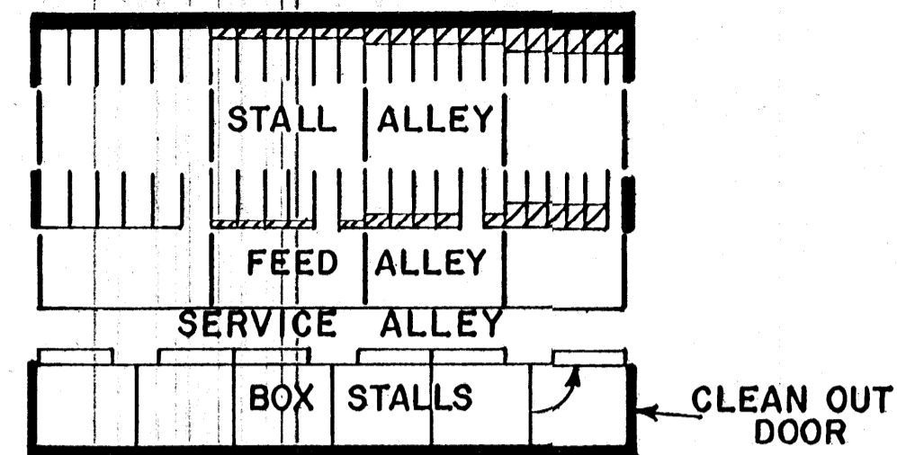
FIG. 2 - BARN 52' WIDE WITH BOX STALLS
