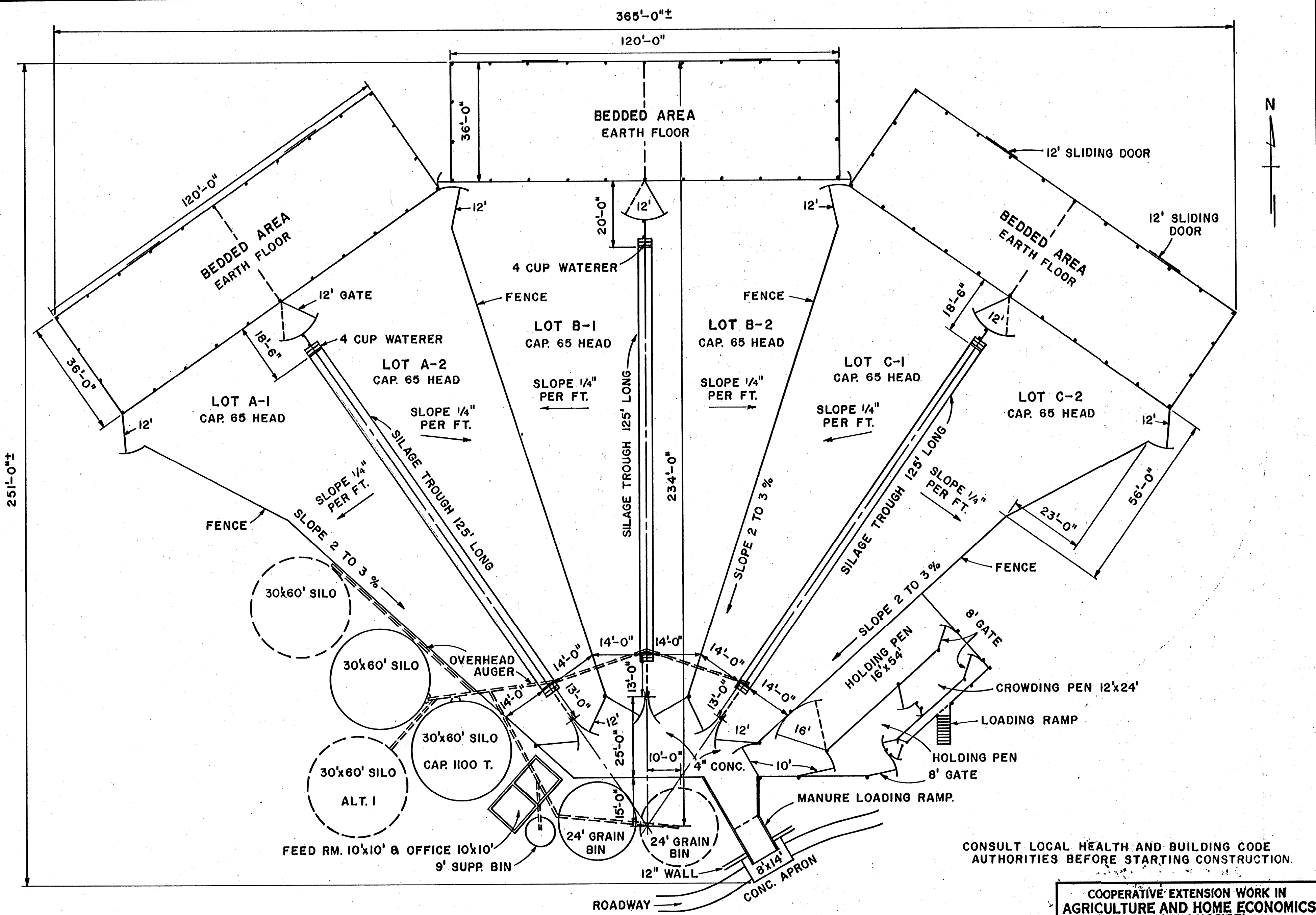
PLAN OF FEED LOTS SCALE: 1" = 20' 10' 5' 0 10' 20' 30'
