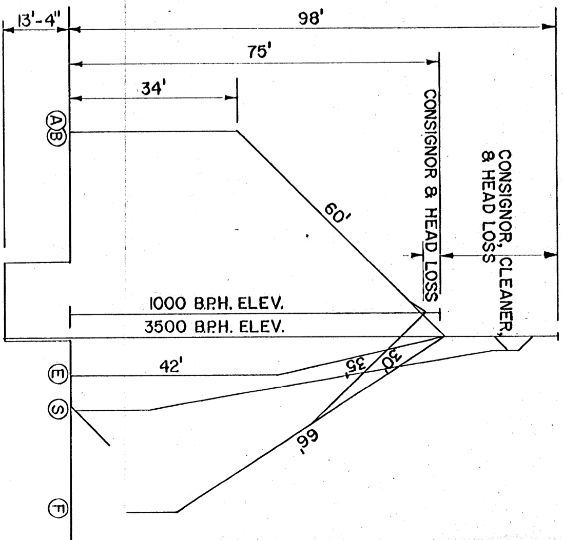
TRUE LENGTH LAYOUT
